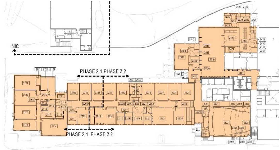
2 PHASE 2 -LEVEL 2 - OVERALL FLOOR PLAN NEW WORK 1" = 3/32"
